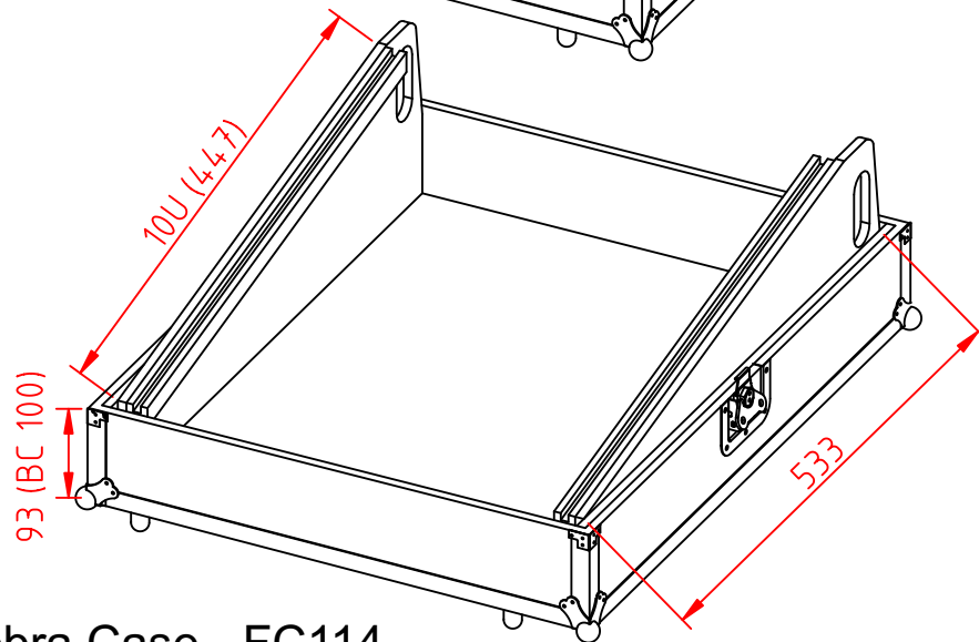
Cobra Case - FC114 10U Mixer Flight Case Material: Plywood Dimensions in mm, may vary slightly
